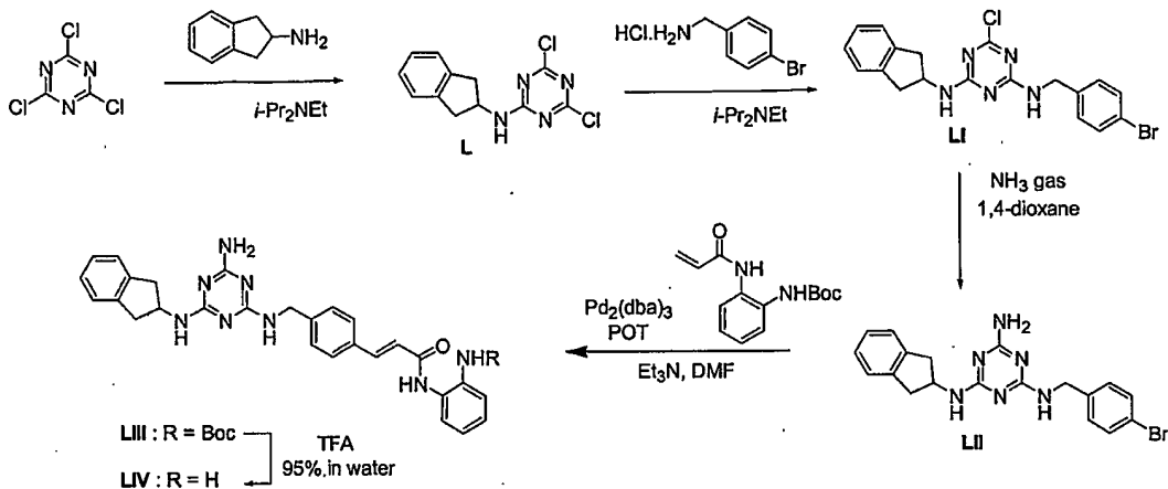
Scheme 9
